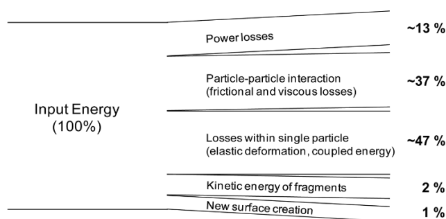
Fig. 8. Rock Crushing and Mineral Grinding Operations have Very Low Energy Efficiency (The data shown corresponds to a ball mill for cement manufacturing. Energy efficiency can be as low as 1%. data from Beke (1964).)
