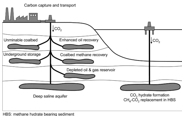
Fig. 7. Carbon Capture and Geological Sequestration (Alternative formation)
