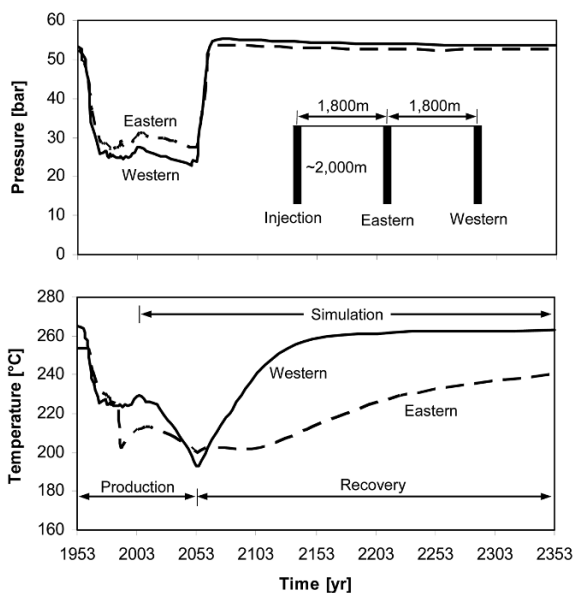
Fig. 5. Pressure and Temperature Recovery in Geothermal Reservoir (Geothermal energy is a resource that can be temporarily depleted. Long recovery times are required afterwards. The data show pressure and temperature evolution at the Wairakei-Tauhara system in two borefields. The values from 1953 to 2003 were measured during operation, and the values from 2004 to 2053 were estimated assuming a constant production level (2003 to 2053) and full recovery (2053 to 2353). Modified from O'Sullivan and Mannington (2005).)
