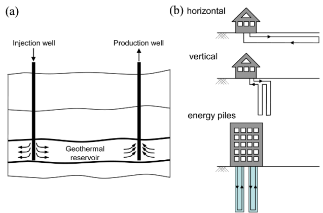
Fig. 4. Geothermal Systems: (a) Deep Geothermal Recovery for Electricity Generation, (b) Distributed Geothermal Storage/Recovery Systems at Shallow Depth for Residential Purposes
