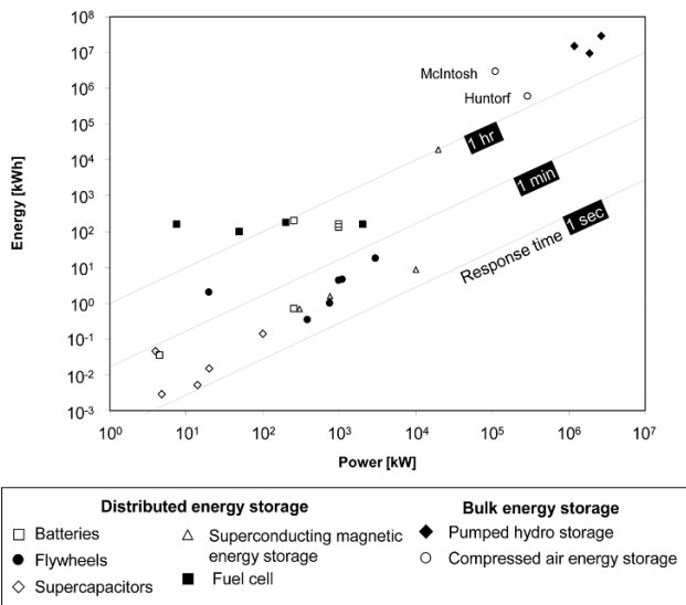
Fig. 6. The Relation between Energy Capacity and Power in Energy Storage Systems (Energy storage systems must satisfy energy capacity and power needs. Geo-storage includes pumped hydro storage PHS, compressed air energy storage CAES, and geothermal storage. Note: PHS and CAES show both high energy capacity and power. Data from Schoenung (2001).)
