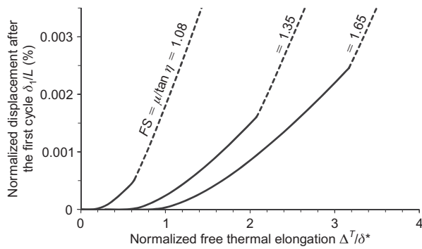
Figure 6. Normalized ratcheting displacement of the membrane upper edge \delta_1/L after the first thermal cycle as a function of the normalized free thermal elongation \Delta T/\delta^* and various static factors of safety FS = \mu/\tan\eta . Dotted lines indicate cases with accelerated ratcheting displacement. Note: geomembrane parameters are found in Tables 1 and 2
